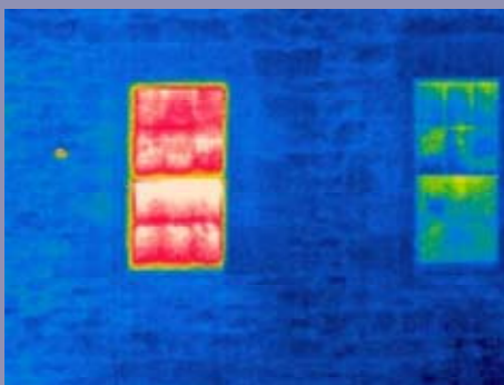
Fig 8. Heat difference from use of shutters. City of Edinburgh Council
