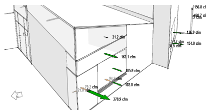
Wind / Stack
