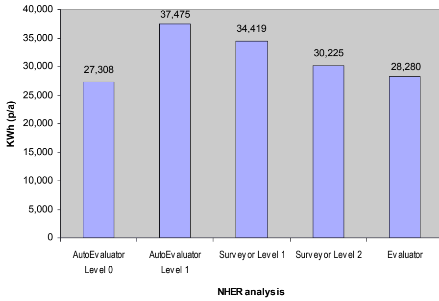
Figure v: Estimated annual energy usage
